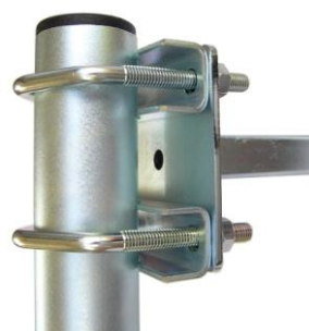
detail uchytenia s 2x VBZ3
