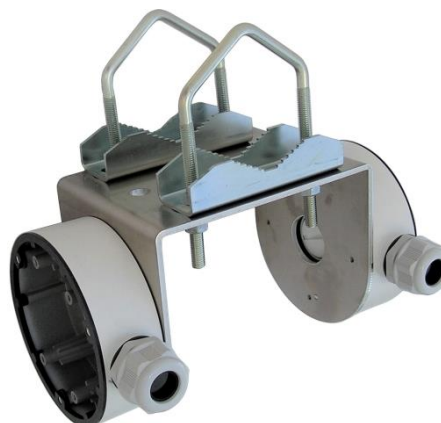
HIK134L + 2x Z85DV85 TWIN + 2x DS-1260ZJ
