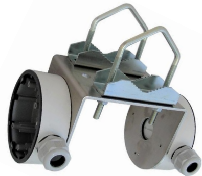
HIK134L + 2x Z85DV85 TWIN + 2x DS-1280ZJ-DM46
